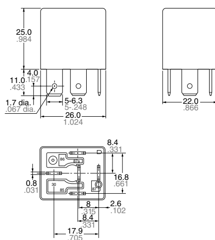
External dimensions
